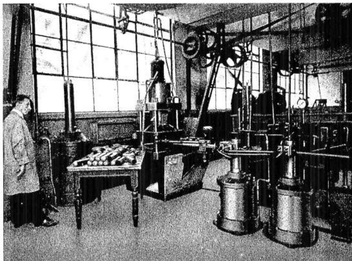
FIGURE 3. Compressors for hydraulic expansion. c. 1935 catalogue (JHPC)
